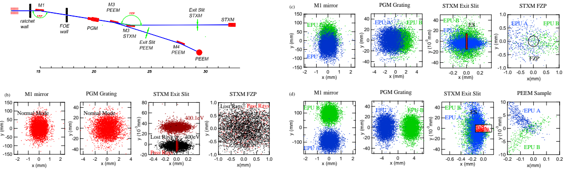
Fig 1. CLS-SM optical layout and ray tracing (400 eV, 500 l/mm, Cff 2.0): (b) STXM in normal operation mode, (c) STXM in 2->1 mode (blue trace from upstream EPU, green from downstream) with 65 \mu rad canting, (d) PEEM in 2->1 250 \mu rad mode. Exit slit (shown as rectangular) corresponds to 4500 resolving power, and single diffraction mode acceptance for STXM.
